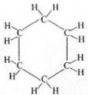
Cyclohexane
