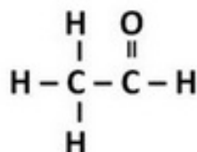
Ethanal
