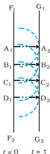
FIGURE 10.3 Huygens geometrical construction for a plane wave propagating to the right. F_1F_2 is the wavefront at t = 0 and G_1G_2 is the wavefront at a later time \tau . The lines A_1A_2 , B_1B_2 ... etc., are normal to both F_1F_2 and G_1G_2 and represent rays.
