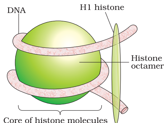
Figure 6.4a Nucleosome
