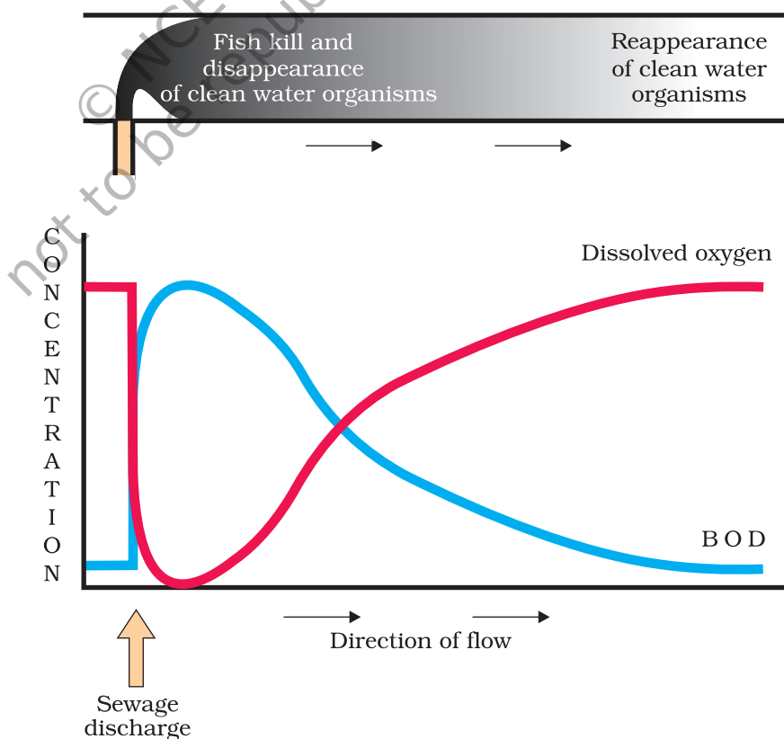
Figure 16.3 Effect of sewage discharge on some important characteristics of a river
