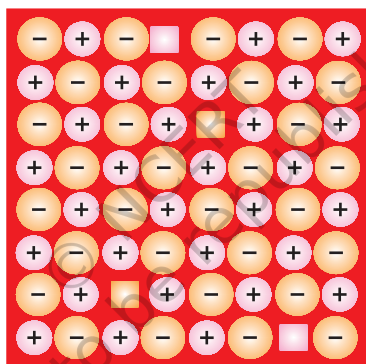
Fig. 1.30: Schottky defects
