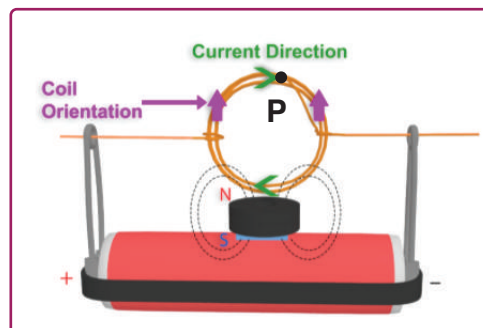
Fig.7.17, Model of a Simple DC Motor
