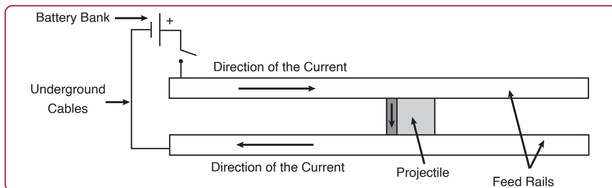
Fig.7.21, Parts of a Railgun
