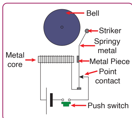
Fig.7.22, Parts of an Electric Bell
