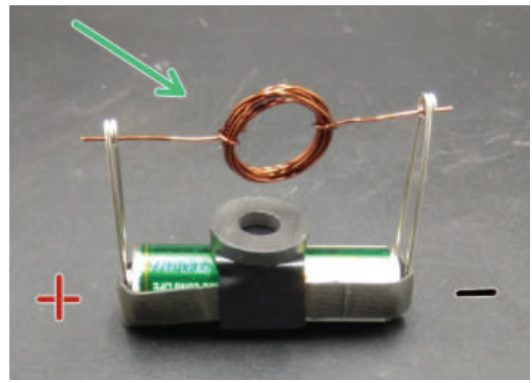
Fig.7.16, Insert the ends of the coil through the "hinge" ends of the safety pins so that the coil aligns directly above the magnets. The coil should spin once you give it a small impetus (push).
