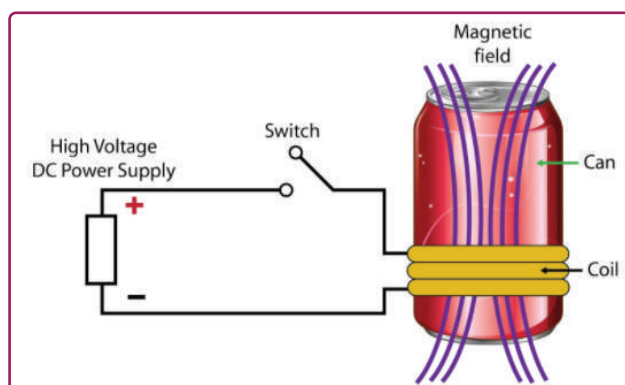
Fig.7.23, A Can Experiment
