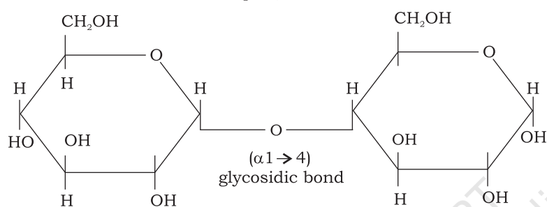
Maltose (α- D-glucopyranosyl-(1 → 4)α-D-glucopyranose)
