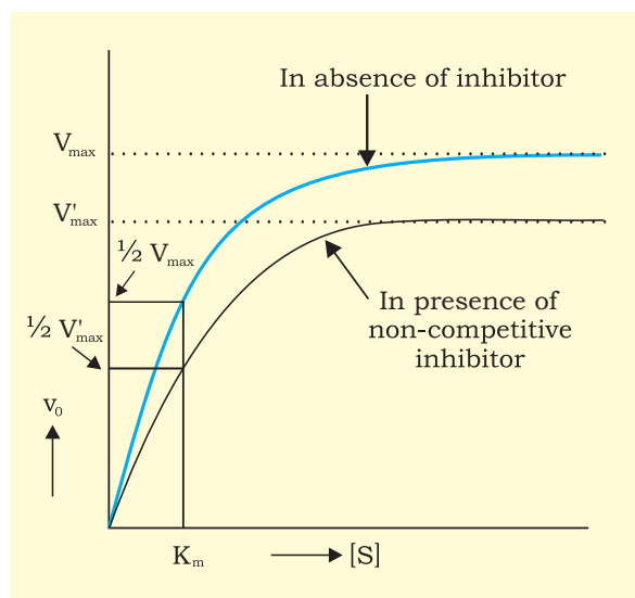
Fig. 4.10: Michaelis Menten plot for non-competitive inhibition
