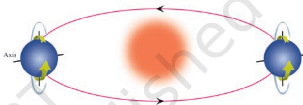
Fig. 17.24 : Uranus in its orbital path
