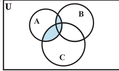
A \cap (B \cup C)
