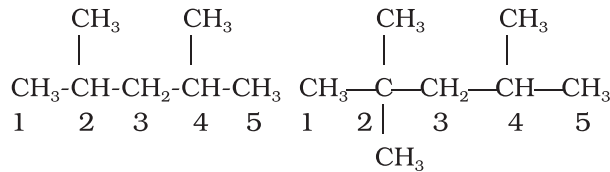
2,4-Dimethylpentane 2,2,4-Trimethylpentane
