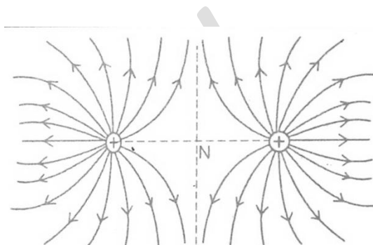
Lines of force due to Two positive charges
