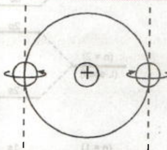
FIGURE 3.26. Spinning of electrons.
