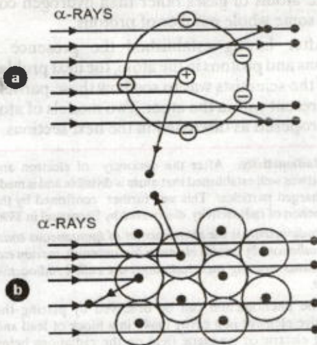
FIGURE 3.9. Scattering of \alpha -particles by (a) a single atom (b) a group of atoms.
