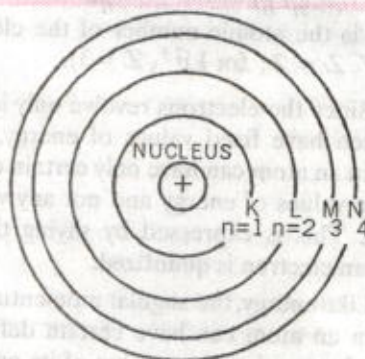
FIGURE 3.21. Circular orbits (energy levels/stationary states) around the nucleus.
