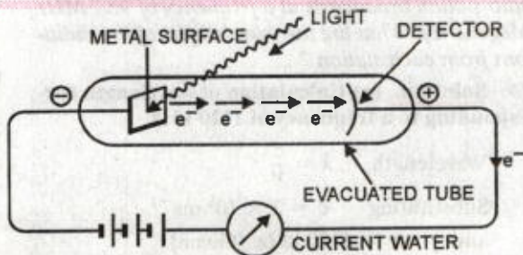
FIGURE 3.14. Apparatus for studying photoelectric effect.
