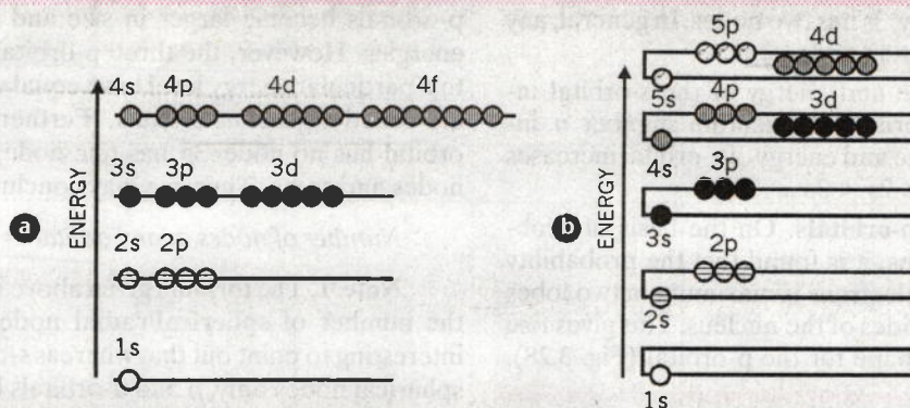
FIGURE 3.30. (a) Energy level diagram for hydrogen atom. (b) Energy level diagram for multielectron atoms.
