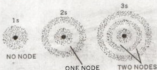
FIGURE 3.27. Shapes of 1s, 2s and 3s orbitals.
