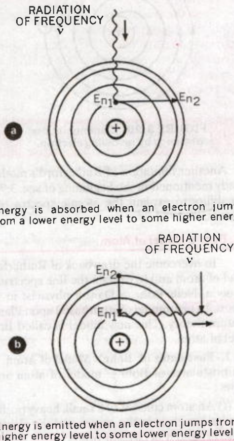
FIGURE 3.22. Energy changes during electronic jumps.
