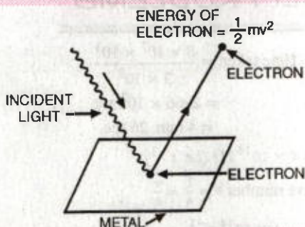
FIGURE 3.13. Photoelectric effect.
