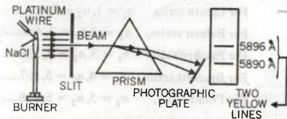
FIGURE 3.17(a). Line spectrum produced from a volatile salt placed in a flame.
