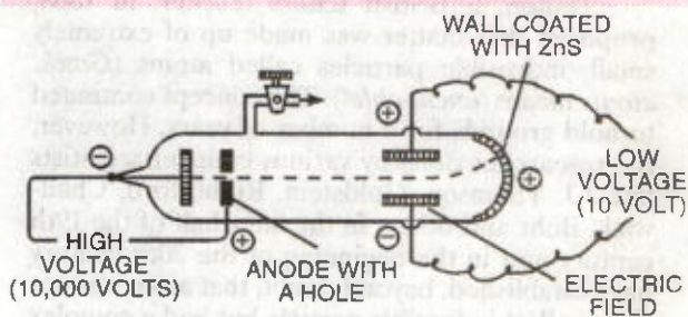
FIGURE 3.4. Deflection of cathode rays towards positive plate of the electric field.
