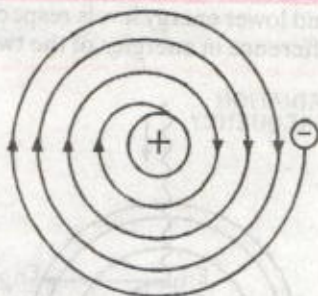
FIGURE 3.20. Continuous loss of energy by revolving electron.
