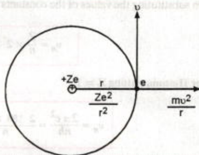
FIGURE 3.33. Bohr's H-like atom.
