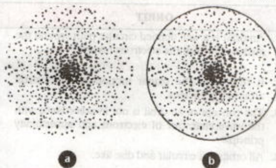
FIGURE 3.24. (a) Electron cloud for the only electron of the hydrogen atom (b) Boundary surface for maximum probability density.
