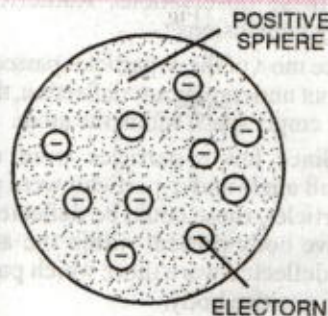
FIGURE 3.7. Thomson model of atom.
