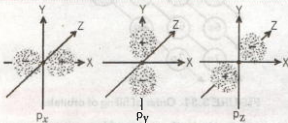
FIGURE 3.29. Different orientations of p-orbitals.
