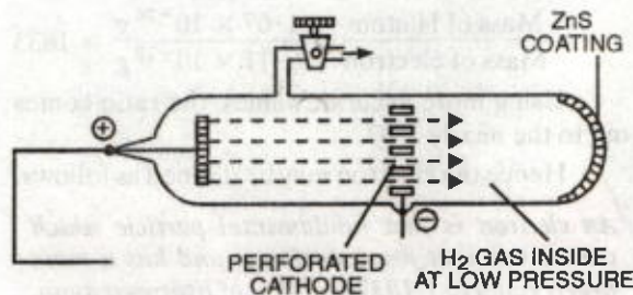
FIGURE 3.5. Production of Anode rays or Positive rays.
