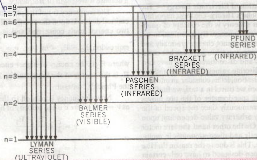
FIGURE 3.23. Different series in the hydrogen spectrum.
