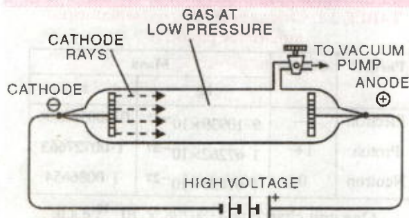
FIGURE 3.1. Discharge tube experiment - Production of cathode rays.
