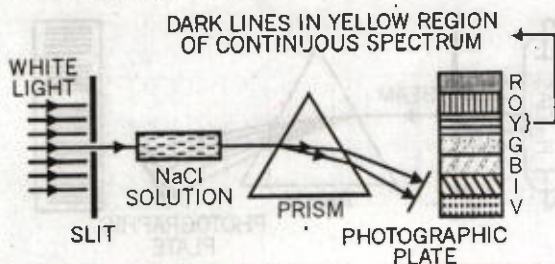
FIGURE 3.18. Production of absorption spectrum.
