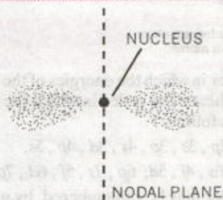
FIGURE 3.28. Shapes of p-orbital.
