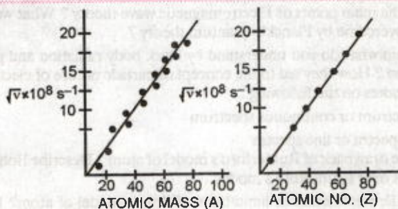
FIGURE 3.32. Plot of \sqrt{\nu} vs A and \sqrt{\nu} vs Z .
