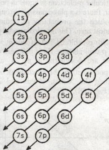
FIGURE 3.31. Order of filling of orbitals.
