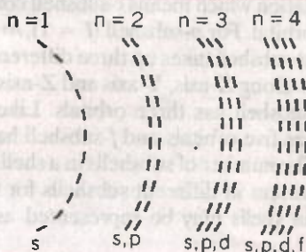
FIGURE 3.25. Sub-shells present in the main shells.
