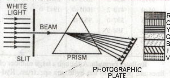
FIGURE 3.16. Continuous spectrum of white light.
