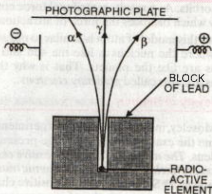
FIGURE 3.6. Effect of electric field on the radiations emitted from a radioactive element.
