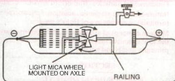
FIGURE 3.3. Rotation of light paddle wheel by cathode rays.
