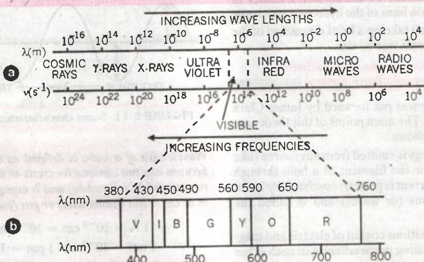
FIGURE 3.12. (a) Complete electromagnetic spectrum (b) Spectrum of visible light.
