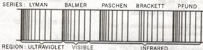
FIGURE 3.19. Emission or atomic spectrum of hydrogen.
