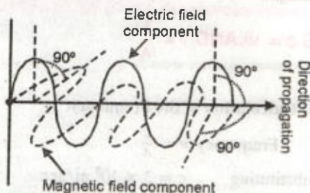
FIGURE. 3.10. Radiation consisting of electric and magnetic fields oscillating in planes perpendicular to each other and both perpendicular to the direction of propagation. They have same wavelength, frequency, speed and amplitude.
