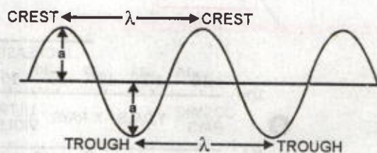
FIGURE 3.11. Some characteristics of a wave.
