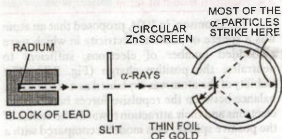
FIGURE 3.8. Rutherford's scattering experiments.
