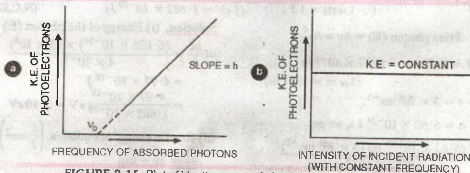
FIGURE 3.15. Plot of kinetic energy of photoelectrons emitted versus (a) frequency of absorbed photons (b) intensity of the incident radiation with constant frequency.
