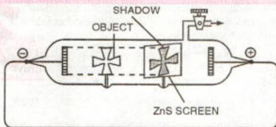
FIGURE 3.2. Production of a shadow of the solid object by cathode rays.
