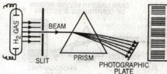
FIGURE 3.17(b). Line spectrum produced from light emitted by discharge tube.
