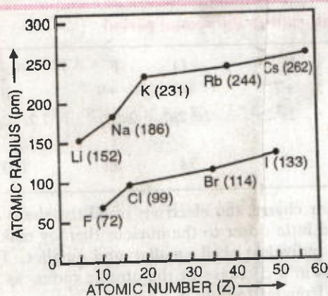
FIGURE 4.9. Variation of atomic radius with atomic number for alkali metals and halogens.
