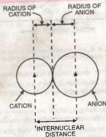
FIGURE 4.10. Internuclear distance and ionic radius.
