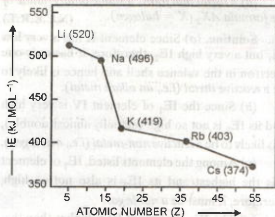
FIGURE 4.4. The variation of first ionization enthalpies with atomic number in group I (alkali metals) of the periodic table.
