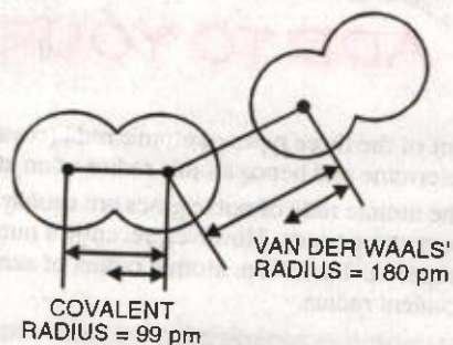
FIGURE 4.6. Covalent and van der Waals' radii of chlorine.
