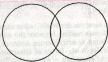
FIGURE 4.7. Overlapping of atomic orbitals to form a covalent bond.
