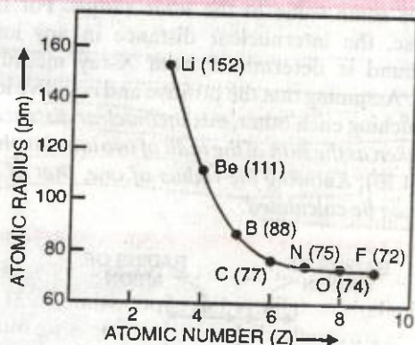
FIGURE 4.8. Variation of atomic radius with atomic number across the second period.
