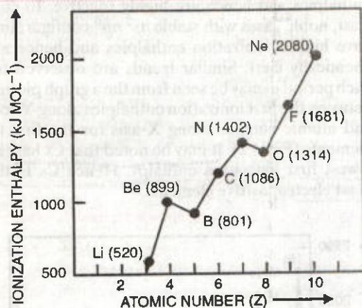
FIGURE 4.3. Variation of first ionization enthalpy with atomic number in second period.
