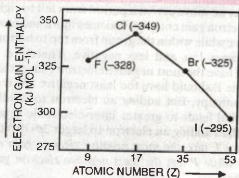
FIGURE 4.5. Variation of electron gain enthalpies of halogens.
