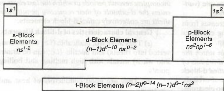
Division of periodic table into s, p, d- and f-blocks.
