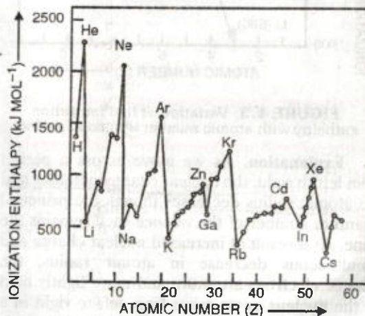
FIGURE 4.2. Variation of first ionization enthalpies of elements with atomic numbers 1 to 60.
