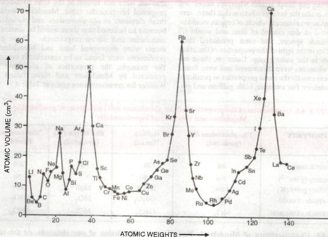
FIGURE 4.1. Lothar Meyer's atomic volume curves.
