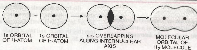
FIGURE 6.9. Formation of H 2 molecule (s-s overlapping).
