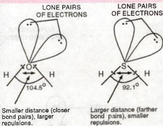
FIGURE 6.42. Repulsion of bond pairs and lone pairs.
