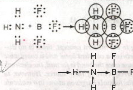
FIGURE 6.43. Formation of a co-ordinate bond between NH 3 and BF 3 .
