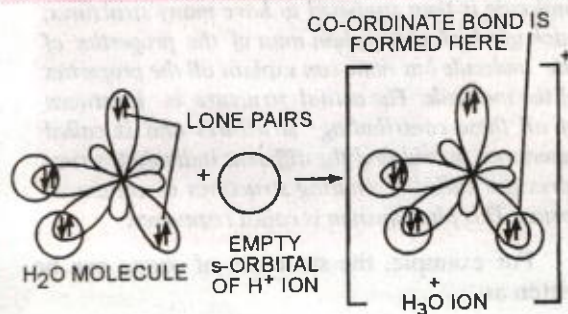
FIGURE 6.47. Formation of \text{H}_3\text{O}^+ ion (orbital concept).
