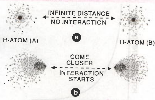
FIGURE 6.4. (a) No interactions at large distances (b) Interactions start as atoms come closer.
