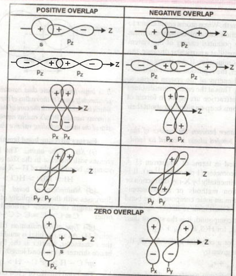
FIGURE 6.17. Depiction of positive, negative and zero overlap.
