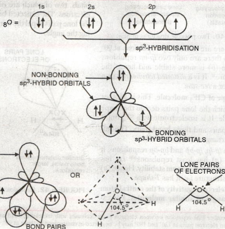
FIGURE 6.39. Formation of water ( \text{H}_2\text{O} ) molecule.
