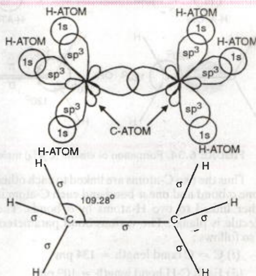
FIGURE 6.33. Formation of ethane molecule.
