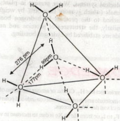
FIGURE 6.51. Each \text{H}_2\text{O} molecule linked to four \text{H}_2\text{O} molecules tetrahedrally.
