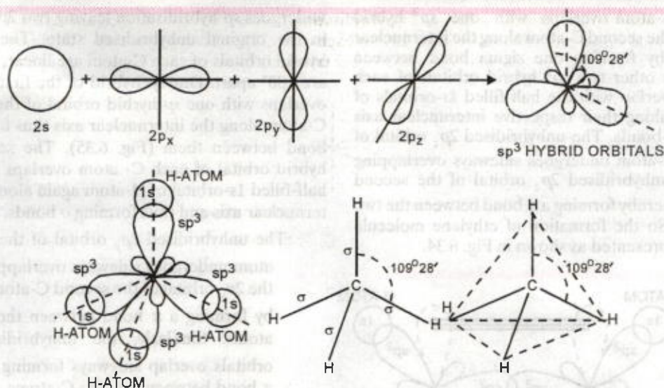
FIGURE 6.32. Formation of \text{CH}_4 molecule.
