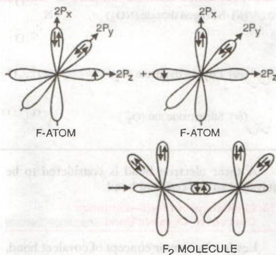
FIGURE 6.3. Formation of Fluorine Molecule.
