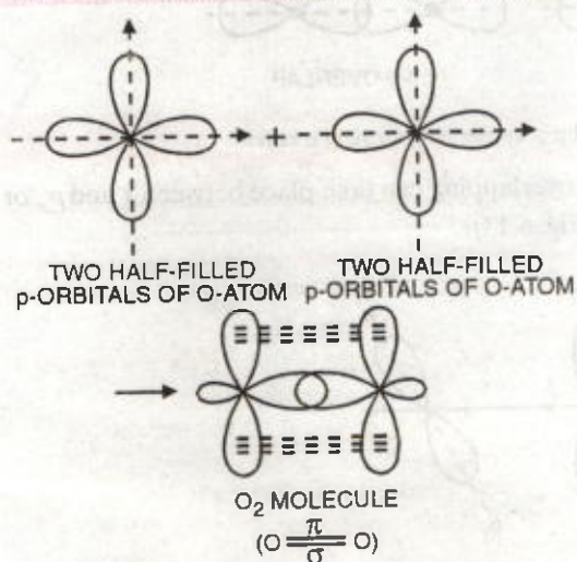
FIGURE 6.15. Formation of oxygen molecule.
