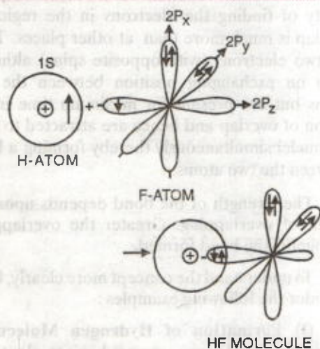
FIGURE 6.2. Formation of HF molecule.
