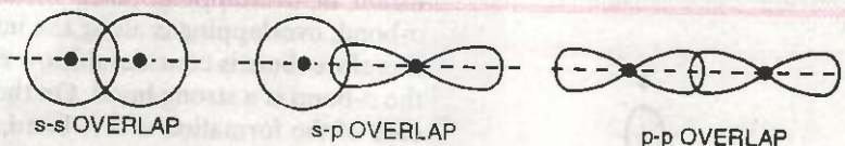
FIGURE 6.12. Representation of s-s, s-p and p-p overlapping forming \sigma bonds.
