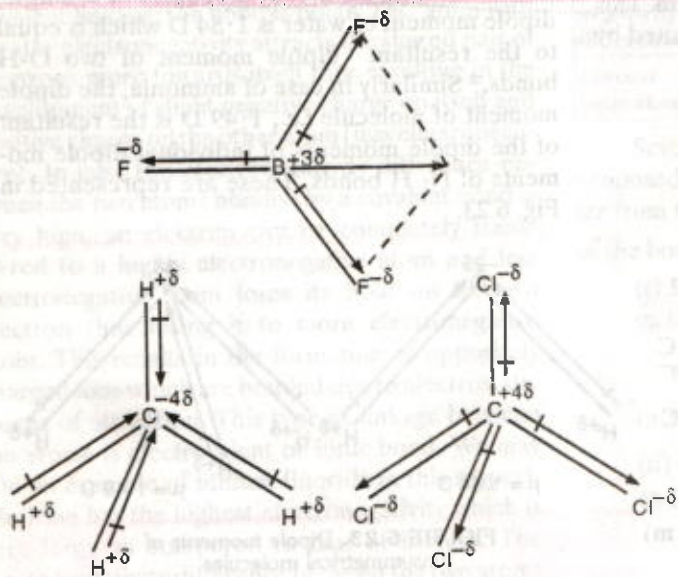
FIGURE 6.25. Dipole moments of zero for symmetrical molecules.
