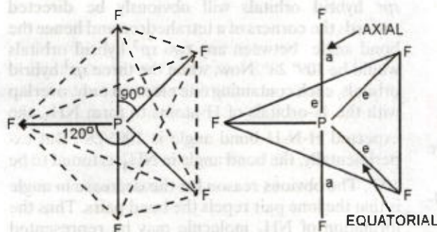
FIGURE 6.36. Trigonal bipyramidal geometry of \text{PF}_5 .
