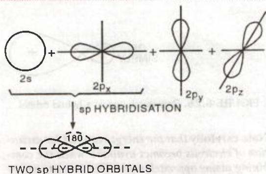
FIGURE 6.27. Diagonal or sp hybridization.
