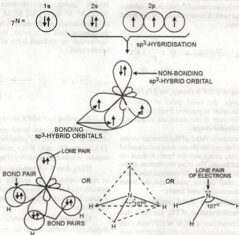
FIGURE 6.38. Formation of ammonia ( \text{NH}_3 ) molecule.
