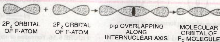
FIGURE 6.11. Formation of F 2 molecule (p-p overlapping).
