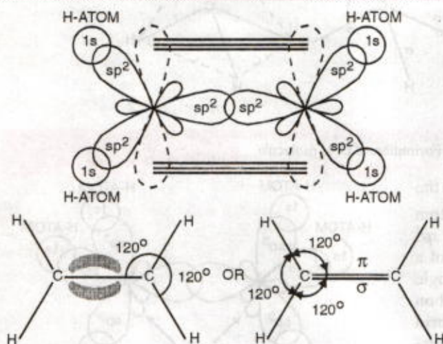
FIGURE 6.34. Formation of ethene ( C_2H_4 ) molecule.
