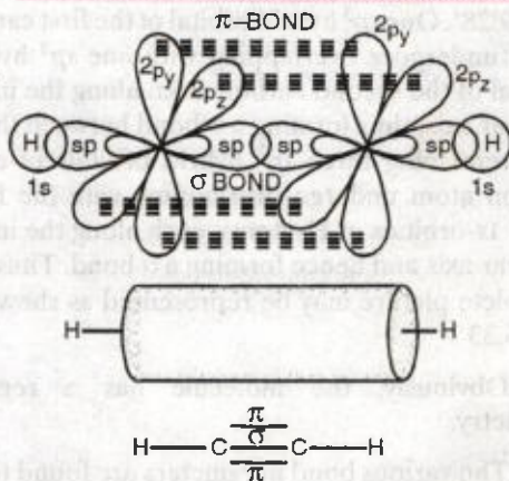
FIGURE 6.35. Formation of acetylene ( C_2H_2 ) molecule (cylindrical shape).
