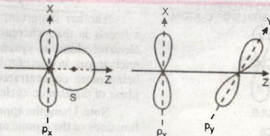
FIGURE 6.13. No overlapping is possible between p_x and s orbitals and between p_x and p_y orbitals
