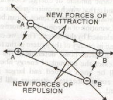
FIGURE 6.5. New forces of attraction and repulsion between two H-atoms approaching each other.
