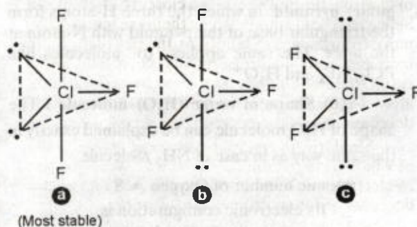
FIGURE 6.41. Three possible structures of ClF_3 .
