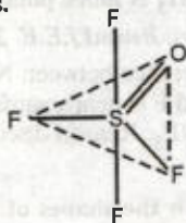
Trigonal bipyramidal ( sp^3d hybridisation)
