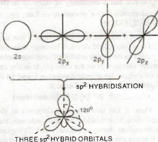
FIGURE 6.28. Trigonal or sp^2 hybridization.
