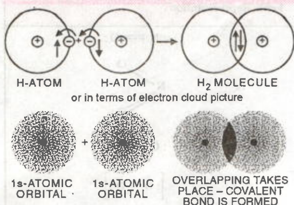
FIGURE 6.1. Formation of hydrogen molecule.
