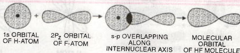
FIGURE 6.10. Formation of HF molecule (s-p overlapping).
