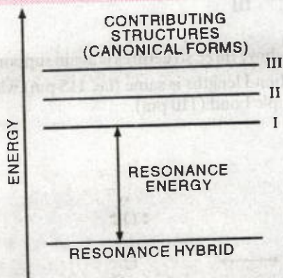
FIGURE 6.48. Concept of resonance energy.
