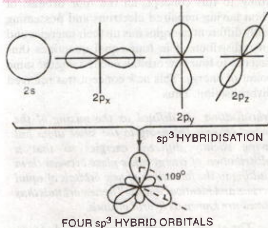
FIGURE 6.29. Tetrahedral or sp^3 hybridization.
