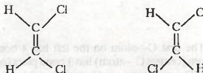
cis-1, 2-dichloro ethene trans-1, 2-dichloroethene
