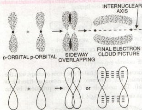
FIGURE 6.14. p-p overlapping forming a pi bond.
