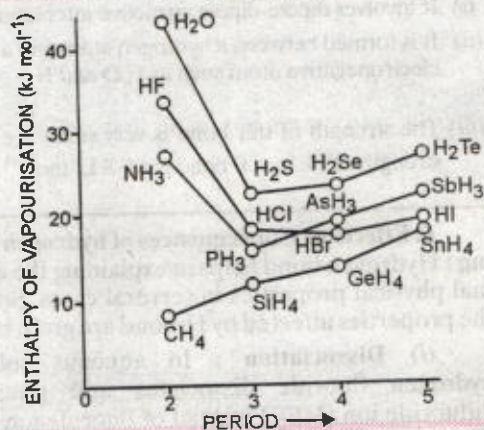
FIGURE 6.49(c). Variation of enthalpies of vaporisation ( \Delta H_{\text{vap}} ) of the hydrides of elements of periods 2 to 5.
