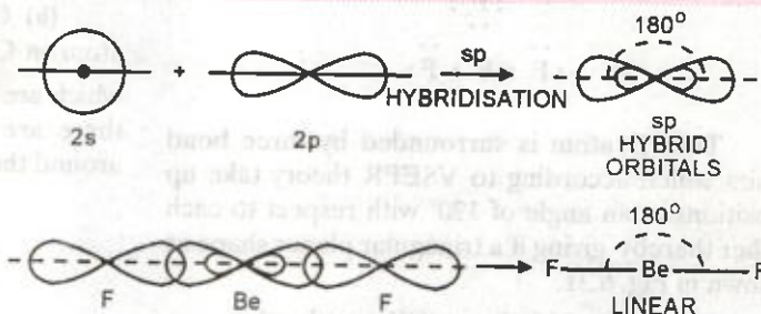
FIGURE 6.30. Formation of sp hybrid orbitals and shape of \text{BeF}_2 .
