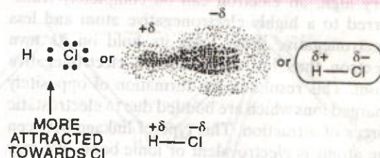
FIGURE 6.19. Polar covalent bond in HCl.
