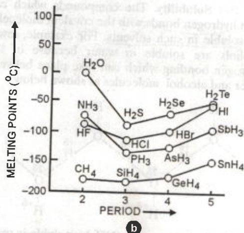
FIGURE 6.49. The abnormally high m.p. and b.p. of \text{H}_2\text{O} , \text{NH}_3 and \text{HF} .*
