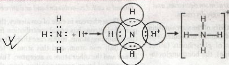
FIGURE 6.45. Formation of ammonium ( \text{NH}_4^+ ) ion.
