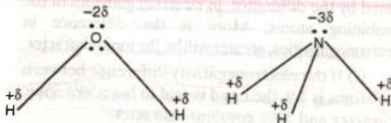
FIGURE 6.21. Polar molecules containing more than one polar bond.
