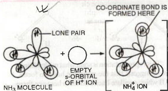
FIGURE 6.46. Formation of \text{NH}_4^+ ion (orbital concept).
