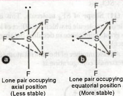
FIGURE 6.40. Two possible structures of SF_4 .
