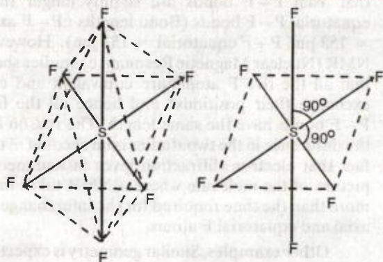
FIGURE 6.37. Octahedral geometry of \text{SF}_6 .
