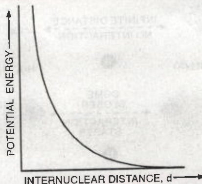
FIGURE 6.8. Variation of potential energy when two helium atoms are brought closer.
