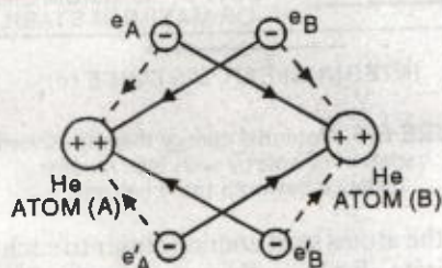
NEW FORCES OF ATTRACTION SHOWN BY SOLID LINES
