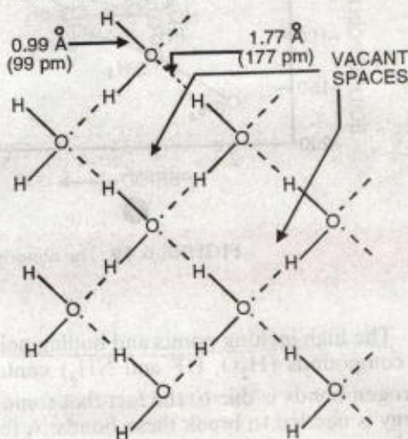
FIGURE 6.50. Cage like structure of \text{H}_2\text{O} in the ice.
