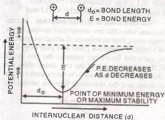
FIGURE 6.6. Potential energy diagram showing variation of energy with internuclear distance between two H-atoms.
