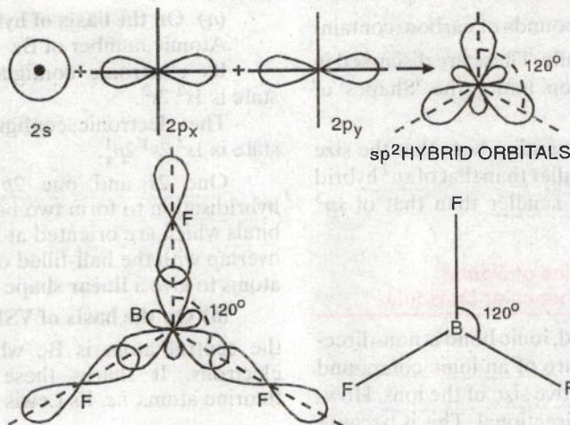
FIGURE 6.31. Formation of sp^2 hybrid orbitals and shape of BF_3 .
