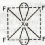
Square planar ( sp^3d^2 hybridisation)
