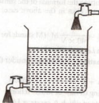
FIGURE 7.9. Rate of inflow = Rate of outflow (level remains constant)
