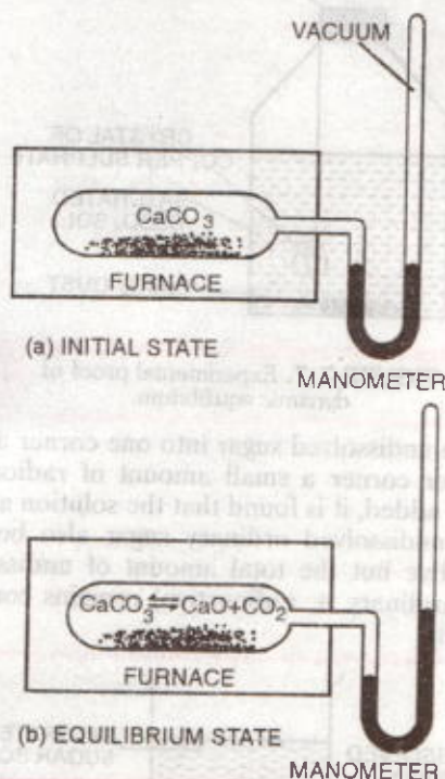
FIGURE 7.5. Equilibrium in the decomposition of \text{CaCO}_3
