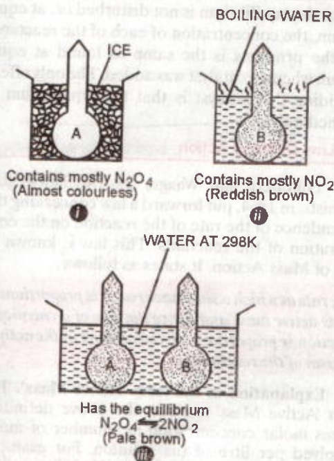
FIGURE 7.10. Equilibrium reaction N_2O_4 \rightleftharpoons 2NO_2 at (i) 273 (ii) 373K and (iii) 298K.
