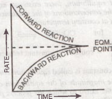
FIGURE 7.4. Variation in reaction rates for the forward and backward reaction with time.
