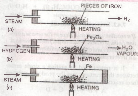
FIGURE 7.3. Reversible reaction occurring in a closed tube (c).
