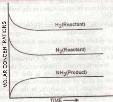
FIGURE 7.6. Representing the attainment of equilibrium for the reaction N_2(g) + 3H_2(g) \rightleftharpoons 2NH_3(g)
