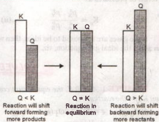
FIGURE 7.11. Direction of shift of reaction depending upon the value of Q as compared with K .
