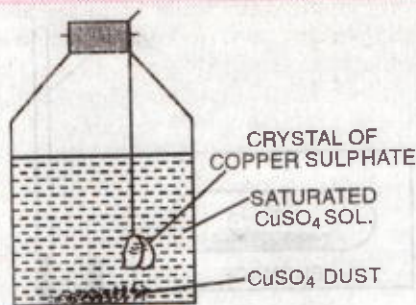
FIGURE 7.7. Experimental proof of dynamic equilibrium.
