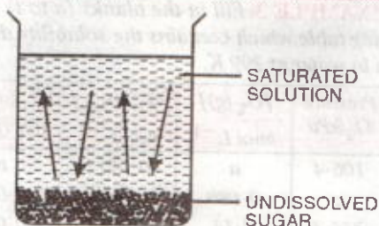
FIGURE 7.2. Equilibrium between undissolved sugar and saturated solution.
