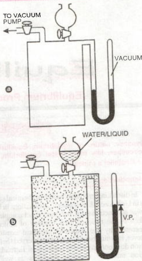
FIGURE 7.1. Method of studying the vapour pressure of a liquid (a) After evacuation (b) After adding the liquid into the evacuated vessel.
