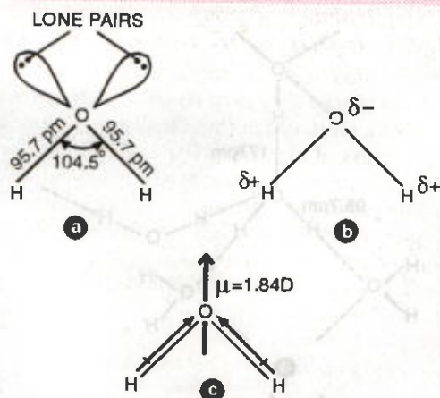
FIGURE 11.6. (a) Structure of \text{H}_2\text{O} in the gas phase (b) Polar nature of \text{H}_2\text{O} molecule (c) Resultant dipole moment of water molecule.
