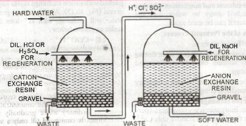
FIGURE 11.9. Ion exchange process involving organic resins.
