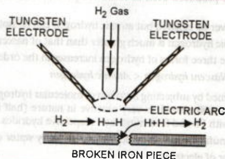
FIGURE 11.14. Atomic Hydrogen Torch.
