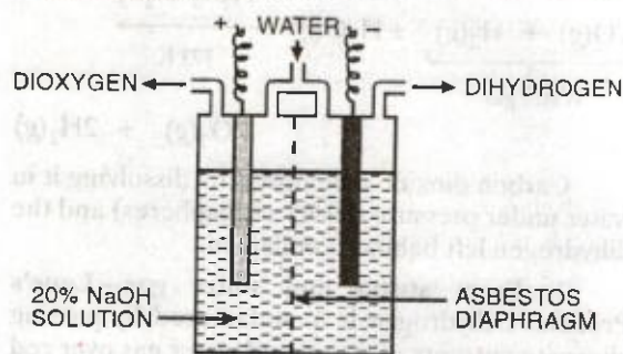
FIGURE 11.4. Electrolysis of water for commercial preparation of dihydrogen.
