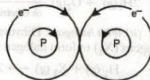
PARA HYDROGEN (Antiparallel nuclear spins ; total nuclear spin = +\frac{1}{2} - \frac{1}{2} = 0 )
