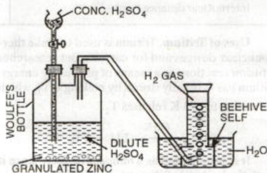
FIGURE 11.2. Preparation of dihydrogen gas in the laboratory.
