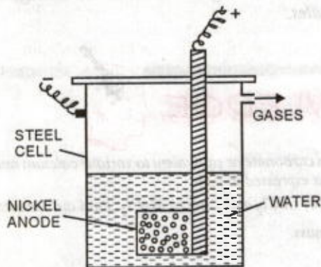
FIGURE 11.10. Electrolytic cell for the preparation of heavy water.
