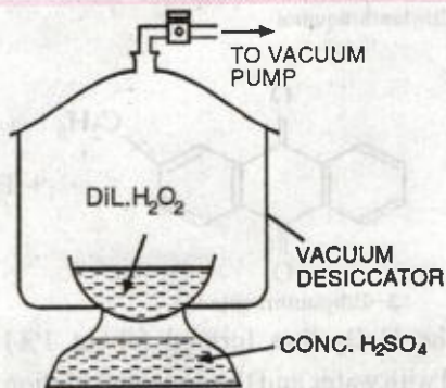
FIGURE 11.12. Vacuum Desiccator.
