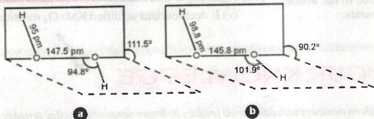
FIGURE 11.13. Structure of H_2O_2 (a) in the gas phase dihedral angle = 111.5^\circ and (b) in the solid phase at 110 K, dihedral angle = 90.2^\circ .
