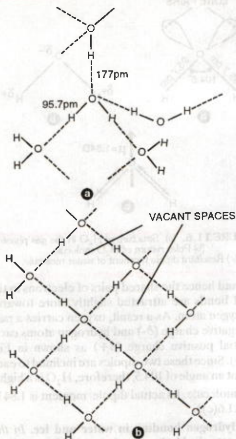
FIGURE 11.7. (a) Structure of water in the liquid state (b) Tetrahedral arrangement of oxygen atoms in ice.
