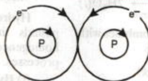
ORTHO HYDROGEN (Parallel nuclear spins ; total nuclear spin = +\frac{1}{2} + \frac{1}{2} = 1 )
