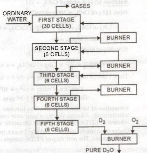
FIGURE 11.11. Flow sheet diagram for the preparation of heavy water by continuous and prolonged electrolysis of water.
