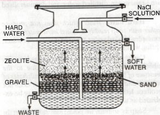
FIGURE 11.8. Permutit process for water softening.
