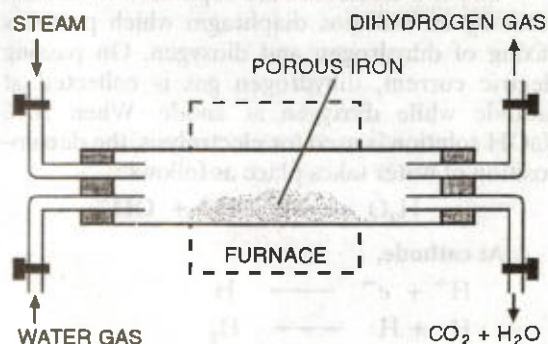
FIGURE 11.3. Manufacture of dihydrogen by Lane's process.
