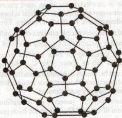
FIGURE 13.11. Buckminster fullerene ( C_{60} ). Note that all carbons are equivalent and that no five-membered rings are adjacent to one another.
