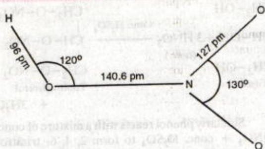
FIGURE 13.17. Structure of nitric acid in the gaseous state.
