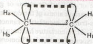
FIGURE 15.16. Restricted rotation about carbon-carbon double bond.
