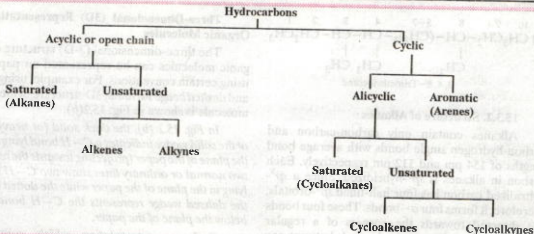
FIGURE 15.1. Classification of hydrocarbons.
