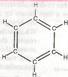
FIGURE 15.21. Kekule structure of benzene.
