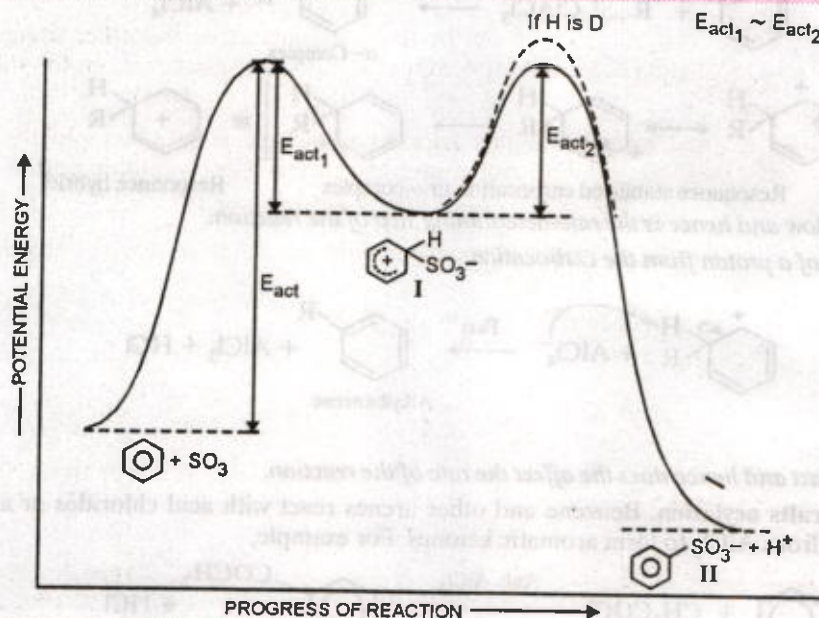
FIGURE 15.29. Some carbocations (I) go to the product, some revert to the starting material. There is some isotope effect, and sulphonation is reversible.
