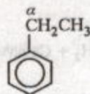
Ethylbenzene [2 \alpha -Hs]
