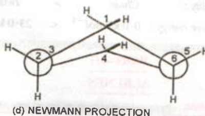
FIGURE 15.14. Sawhorse and Newmann Projections of chair and Boat Conformations of Cyclohexane.
