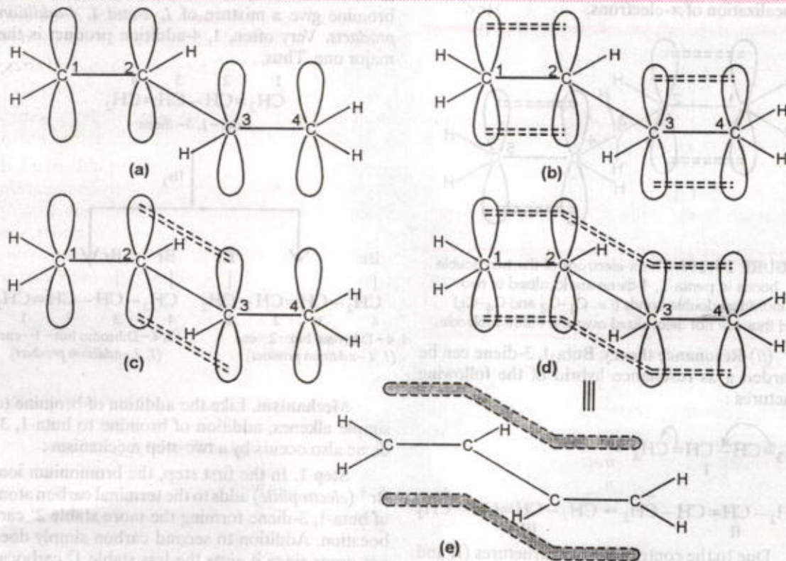
FIGURE 15.19. Orbital picture of buta-1, 3-diene.
