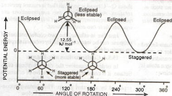
FIGURE 15.9. Variation of energy during rotation about C—C single bond in ethane molecule.
