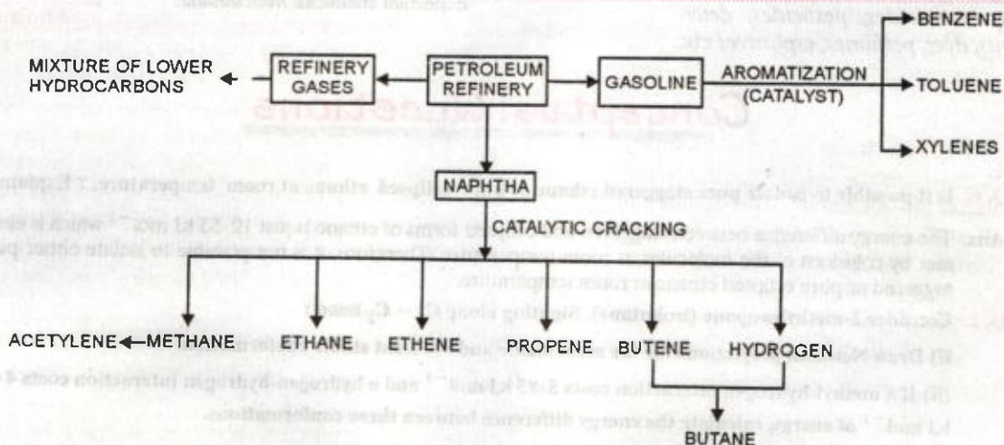
FIGURE 15.31. Hydrocarbons from petroleum refining.
