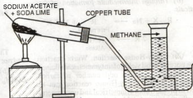
FIGURE 15.3. Laboratory preparation of methane.
