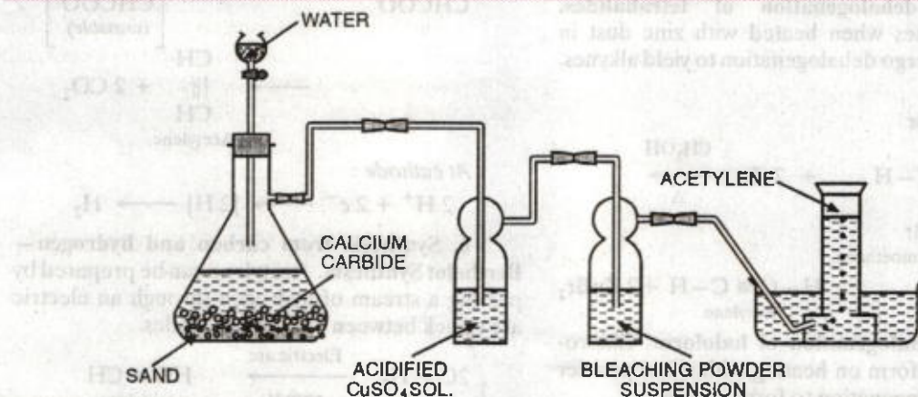
FIGURE 15.18. Laboratory preparation of acetylene.
