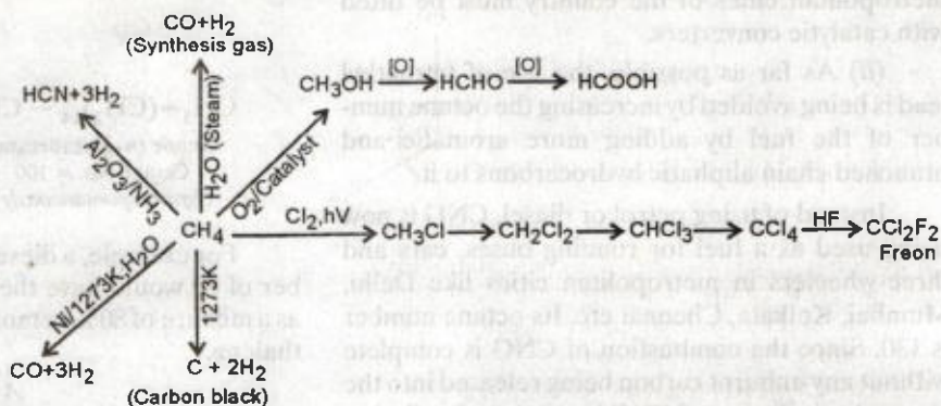
FIGURE 15.32. Industrial preparation of some important chemicals from methane
