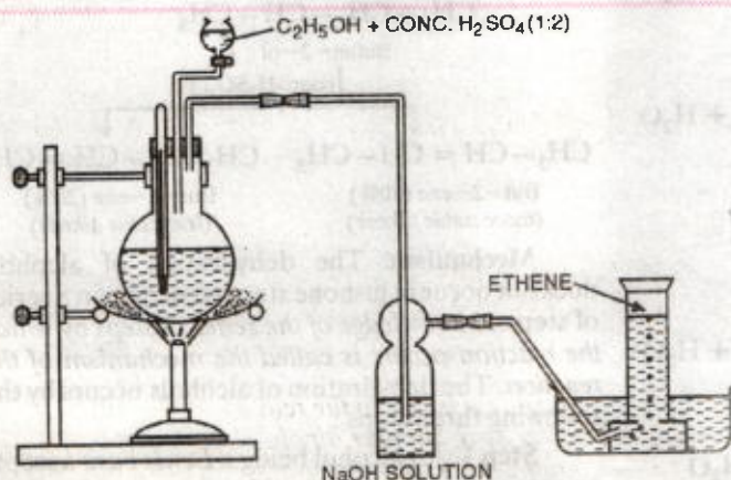
FIGURE 15.17. Laboratory preparation of ethene
