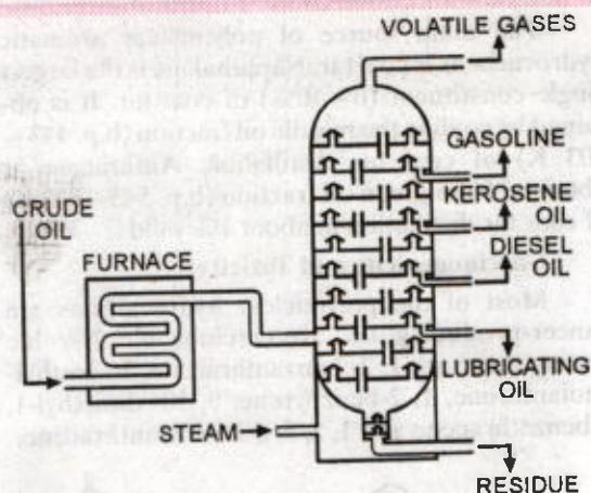
FIGURE 15.30. Fractional distillation of crude oil.
