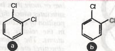
FIGURE 15.22. Kekule isomers of o -dichlorobenzene.
