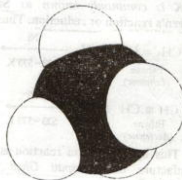
Space Filling Model
