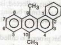
9,10-Dimethyl 1,2-benzanthracene
