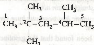
2, 2, 4-Trimethylpentane or Iso-octane (Octane number taken as 100)
