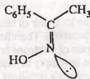
anti -Methyl phenyl ketoxime
