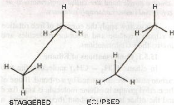
FIGURE 15.7. Sawhorse representation for Staggered and Eclipsed conformations of ethane.
