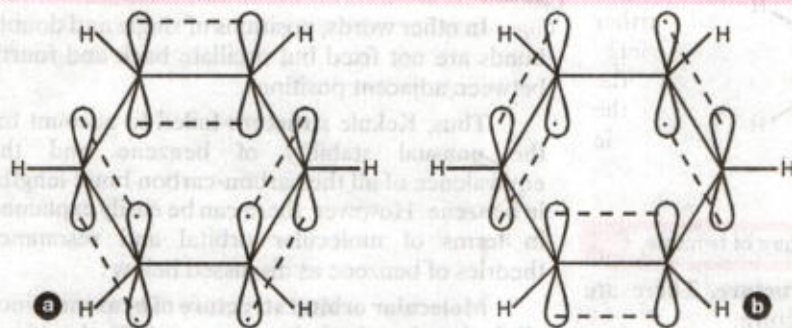
FIGURE 15.25. Two possible sideways overlap of six unhybridized p-orbitals to form three \pi -bonds.
