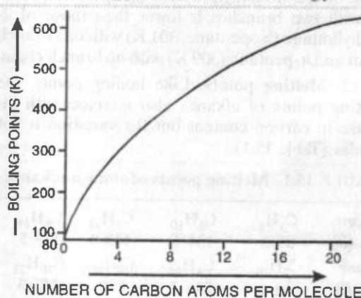
FIGURE 15.4. Increase in the boiling points of n-alkanes with the increase in the number of carbon atoms per molecule of the homologous series.
