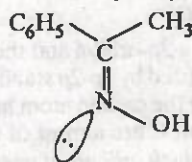
syn -Methyl phenyl ketoxime
