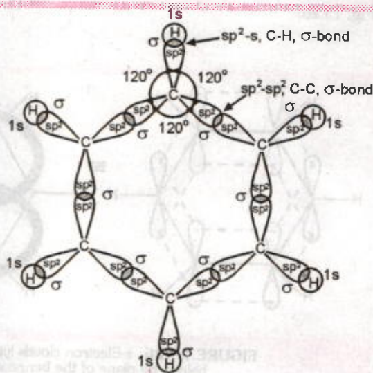
FIGURE 15.24. \sigma -Bond skeleton of benzene.
