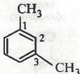
1,3-Dimethylbenzene or m -Dimethylbenzene or m -Xylene
