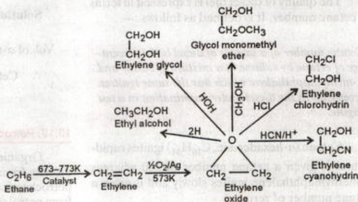
FIGURE 15.33. Industrial preparation of some important chemicals from ethane.
