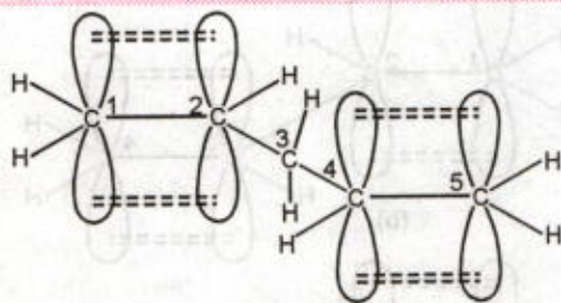
FIGURE 15.19f. The \pi -electrons of the two double bonds in penta-1, 4-diene are localized in two individual double bonds (i.e. C_1 - C_2 and C_4 - C_5 ) and thus are not delocalized over the entire molecule.
