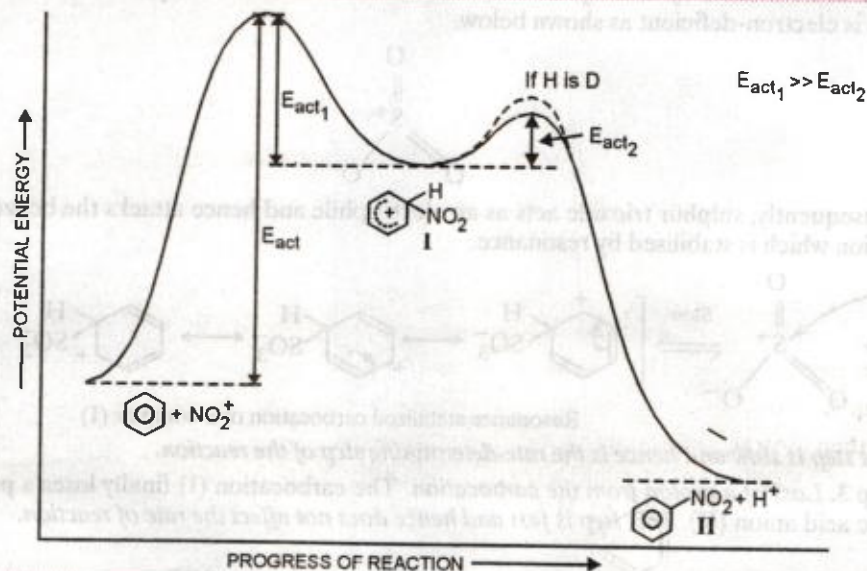
FIGURE 15.28. Formation of carbocation is the rate-determining step ; it occurs equally rapidly whether C-H or C-D bond is to be broken. All the carbocations (I) go to the product (II). There is no isotope effect and nitration is irreversible.
