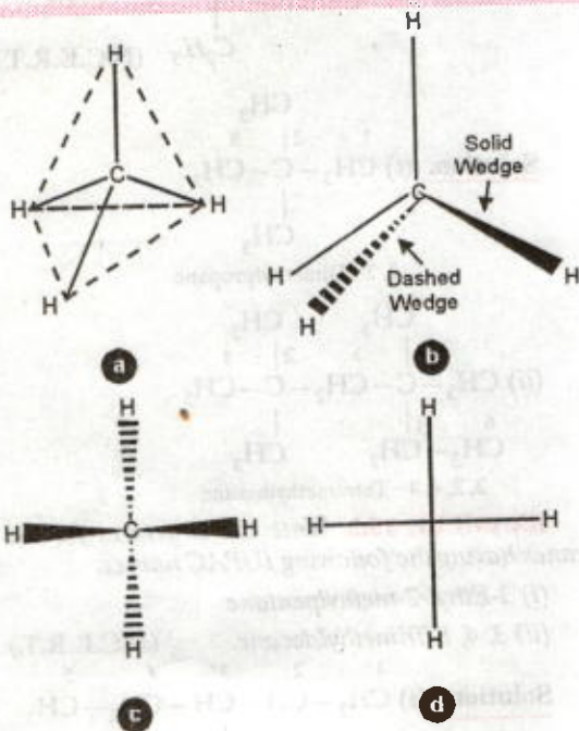
FIGURE 15.2. Representation of methane molecule (a) tetrahedral (b) three-dimensional, i.e., 3D (c) another 3D view (d) two-dimensional, i.e., 2D or Fisher Projection formula.
