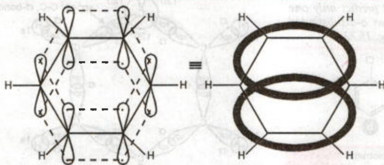
FIGURE 15.26. \pi -Electron clouds lying above and below the plane of the benzene ring.
