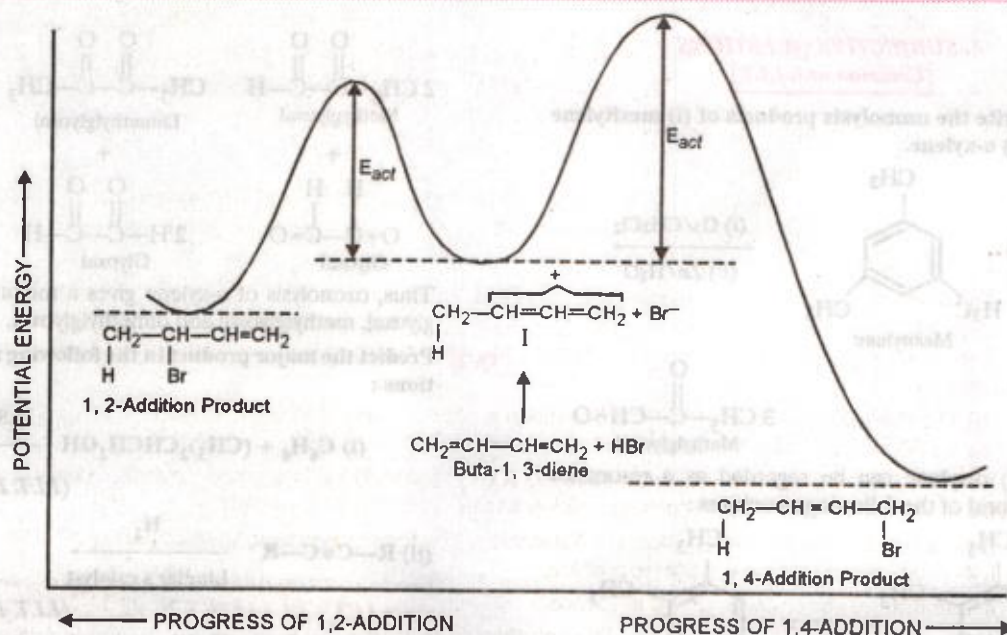
FIGURE 15.34. Potential energy changes during the progress of the reaction : 1, 2-us.-1, 4-addition.
