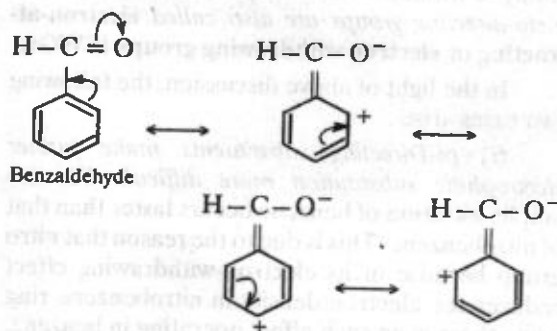
Resonance in benzaldehyde
