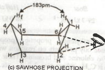
FIGURE 15.14. Sawhorse and Newmann Projections of chair and Boat Conformations of Cyclohexane.
