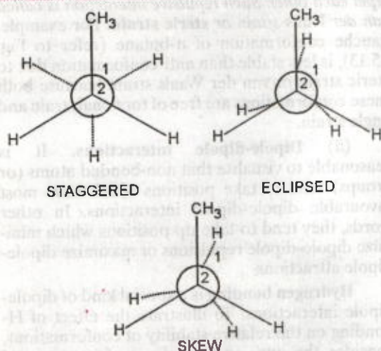
FIGURE 15.10. Newmann projection formulae for staggered, eclipsed and skew conformations of propane.
