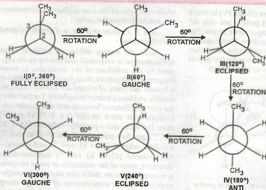
FIGURE 15.11. Newman projections for staggered and eclipsed conformations of n -butane.
