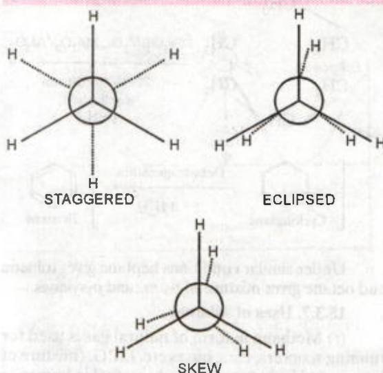
FIGURE 15.8. Newman projection formulae for Staggered, Eclipsed and Skew conformations of ethane.
