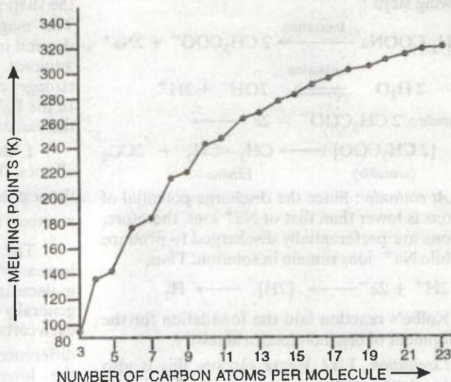
FIGURE 15.5. Increase in the melting points of n -alkanes with the increase in the number of carbon atoms per molecule of the homologous series.
