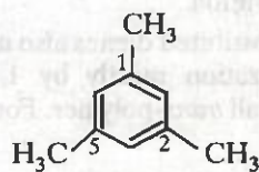
1, 3, 5-Trimethylbenzene (Mesitylene)
