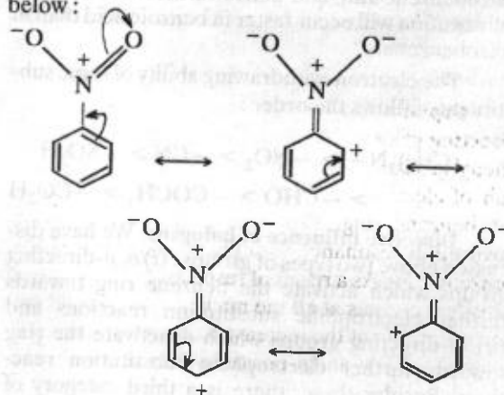
Resonance in nitrobenzene
