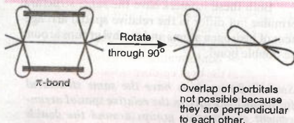
FIGURE 15.15. Rotation about a carbon-carbon double bond.
