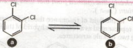
FIGURE 15.23. Dynamic equilibrium between two Kekule isomers of o -dichlorobenzene.
