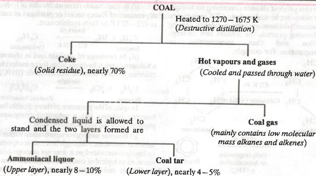
FIGURE 15.20. Flow chart of destructive distillation of coal.
