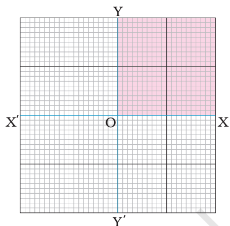
Fig. 13.11 x-axis and y-axis on a graph paper
