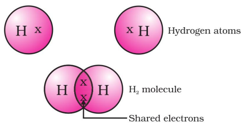
Figure 4.1 A molecule of hydrogen
