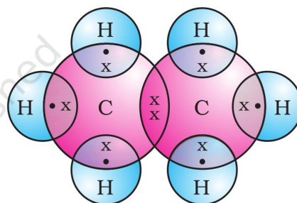
Figure 4.6 (c) Electron dot structure of ethane
