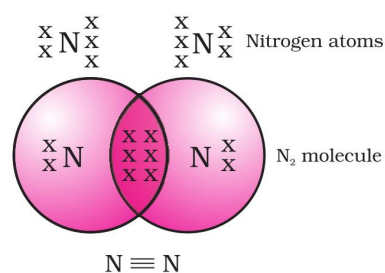
Figure 4.4 Triple bond between two nitrogen atoms
