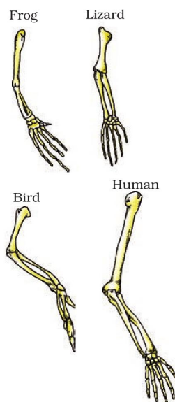
Figure 9.8 Homologous organs
