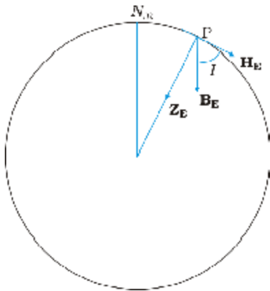
FIGURE 5.10 The circle is a section through the earth containing the magnetic meridian. The angle between B_E and the horizontal component H_E is the angle of dip.
