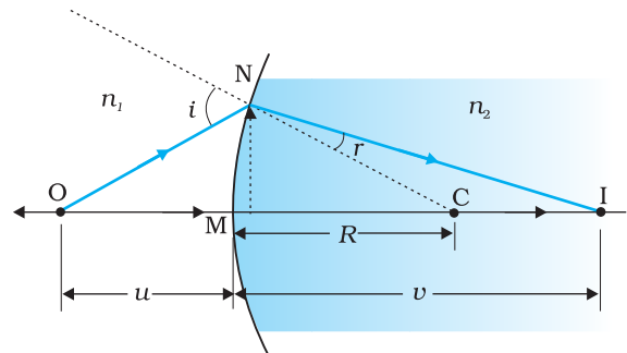
FIGURE 9.17 Refraction at a spherical surface separating two media.
