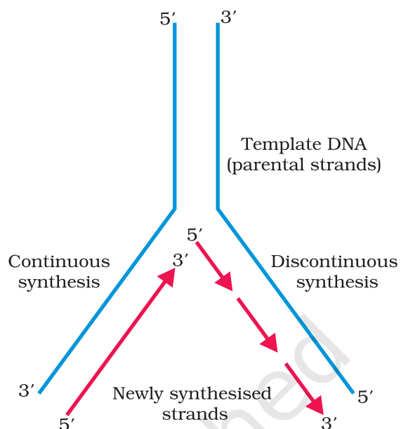
Figure 6.8 Replicating Fork
