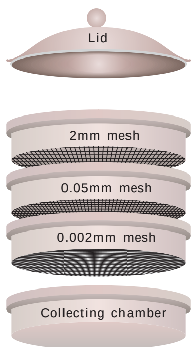
Fig.15.2 Sieve set
