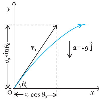
Fig 4.17 Motion of an object projected with velocity v_0 at angle \theta_0 .
