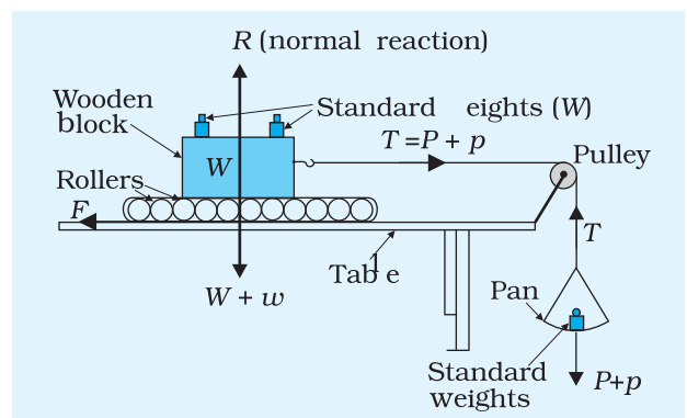
Fig. A 4.1: Setup to study rolling friction
