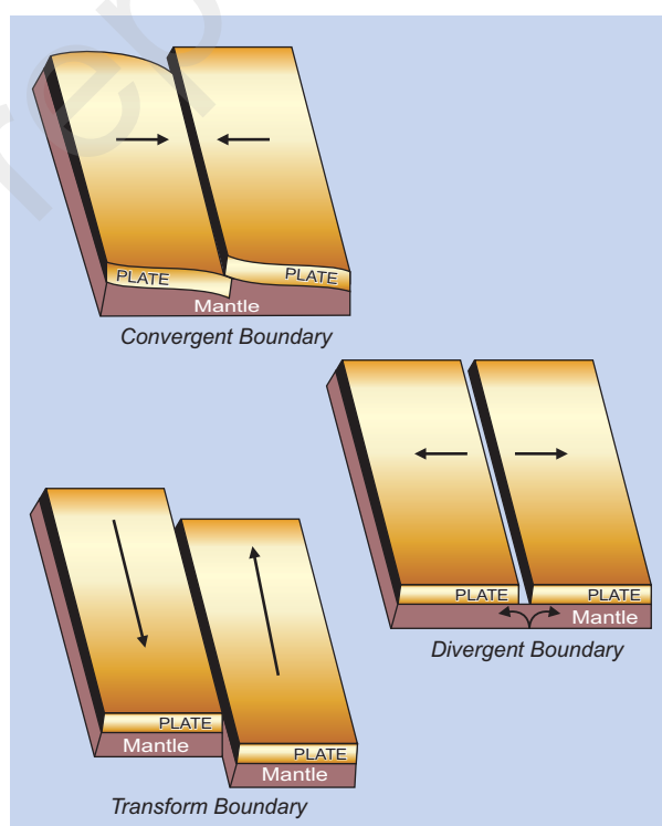
Figure 2.1 : Plate Boundaries
