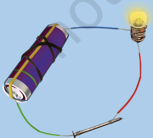
Fig. 4.2 : Electric tester
