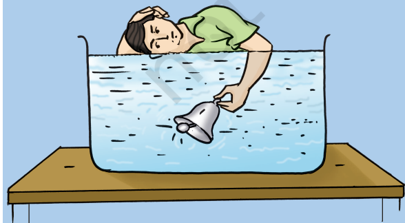
Fig. 13.11 : Sound travelling through water
