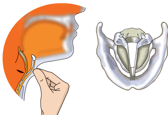
Fig.13.8 : Voice box in humans
