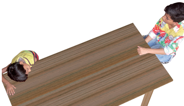
Fig. 13.13 : Sound can travel through solids
