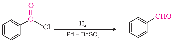
Benzoyl chloride
