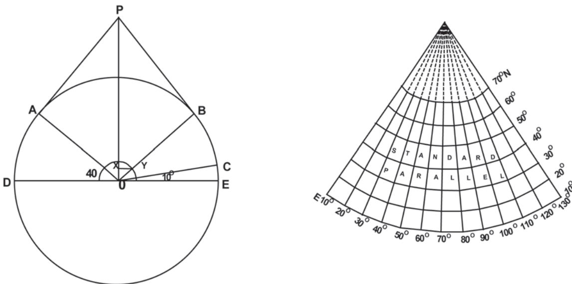
Figure 4.3 Simple Conical Projection with one standard parallel
