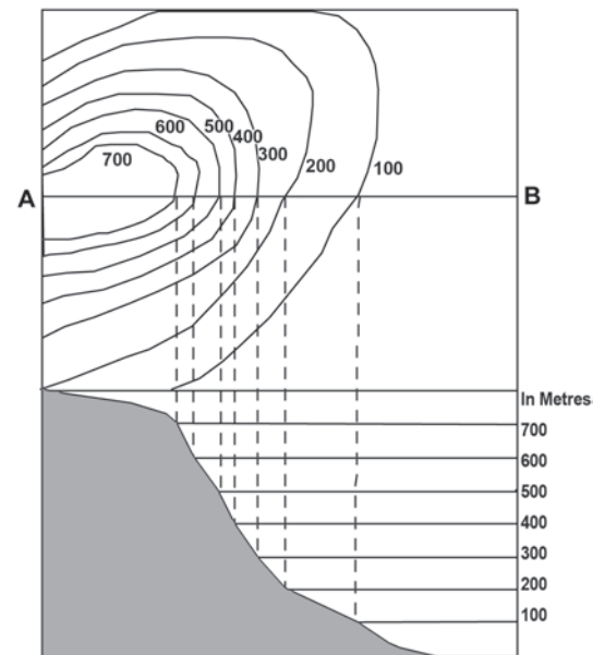
Steep Slope
