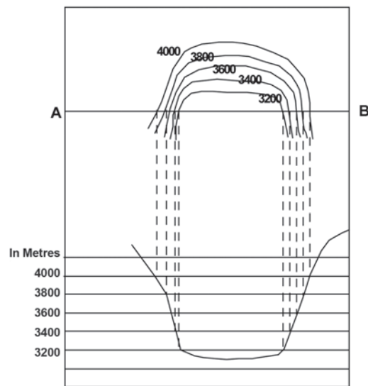
U-Shaped Valley
