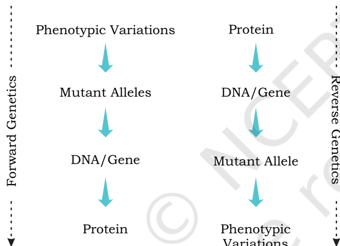
Fig. 6.14: Forward genetics
