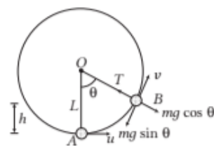
Motion of a particle in vertical circle
