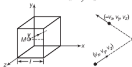
Elastic collision of a gas molecule along x -component of velocity
