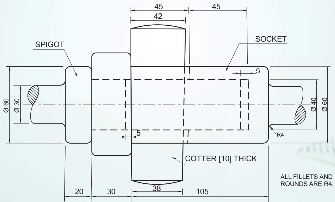
SOCKET AND SPIGOT JOINT
