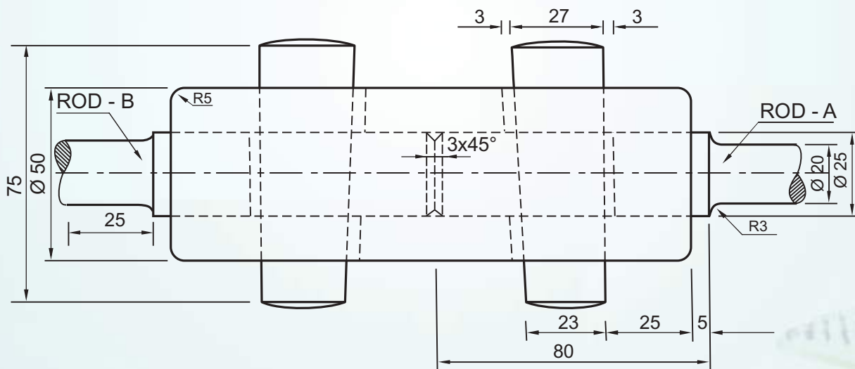
SLEEVE AND COTTER JOINT
