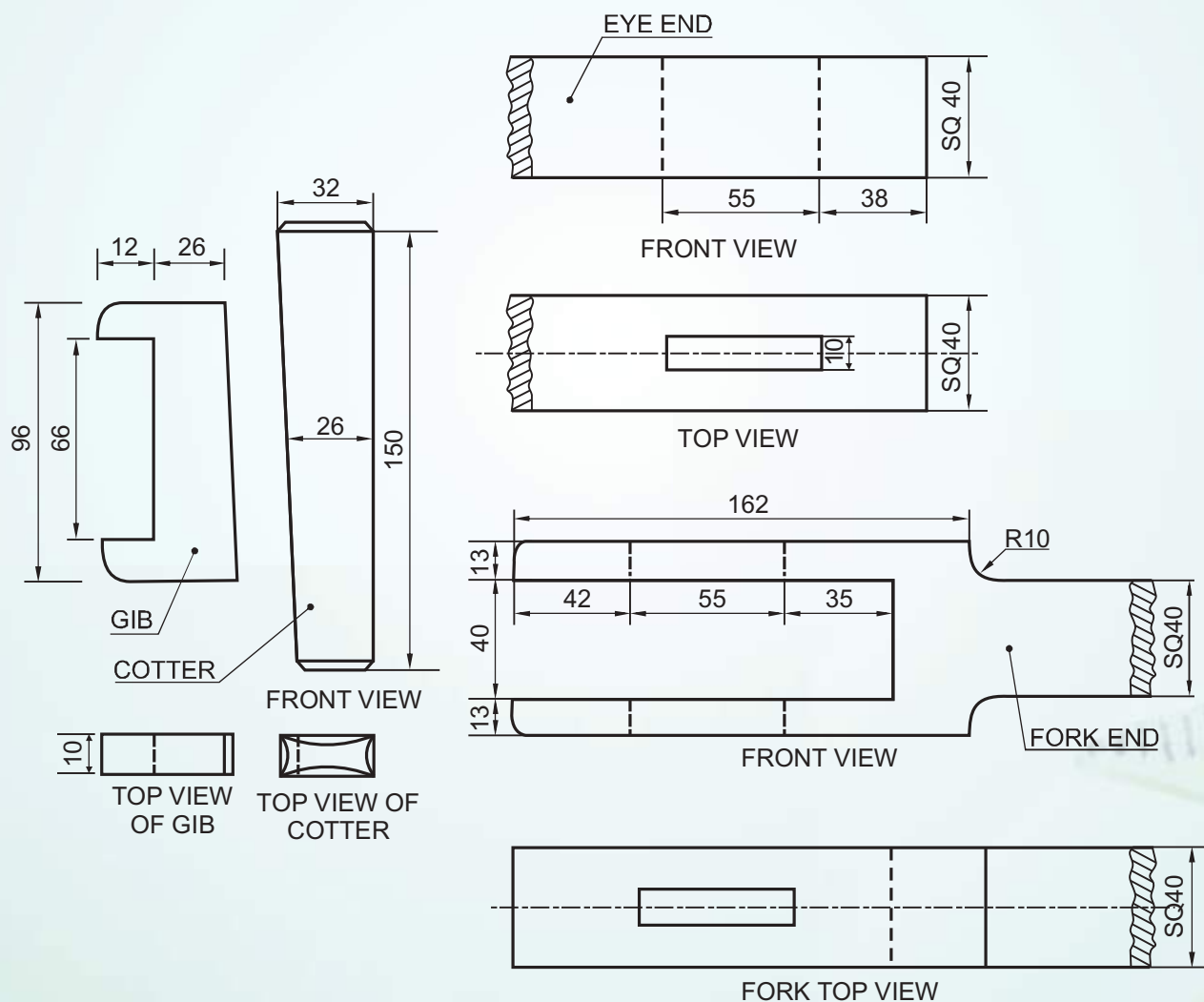
DETAILS OF A GIB AND COTTER JOINT
