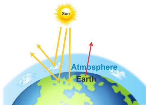
Greenhouse Effect
