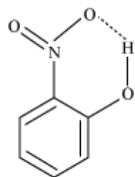
Intramolecular H-bonding in o -Nitrophenol
