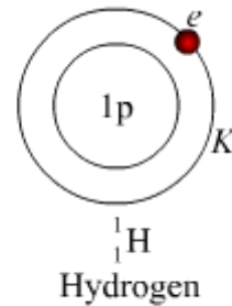
Model of the hydrogen atom
