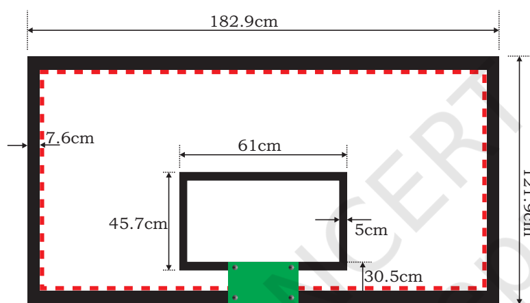
Fig. 5.4: Basketball backboard
