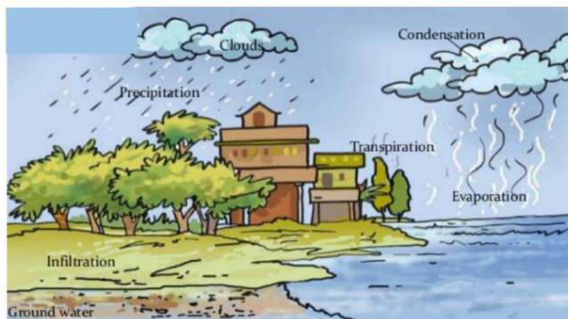
Water Cycle
