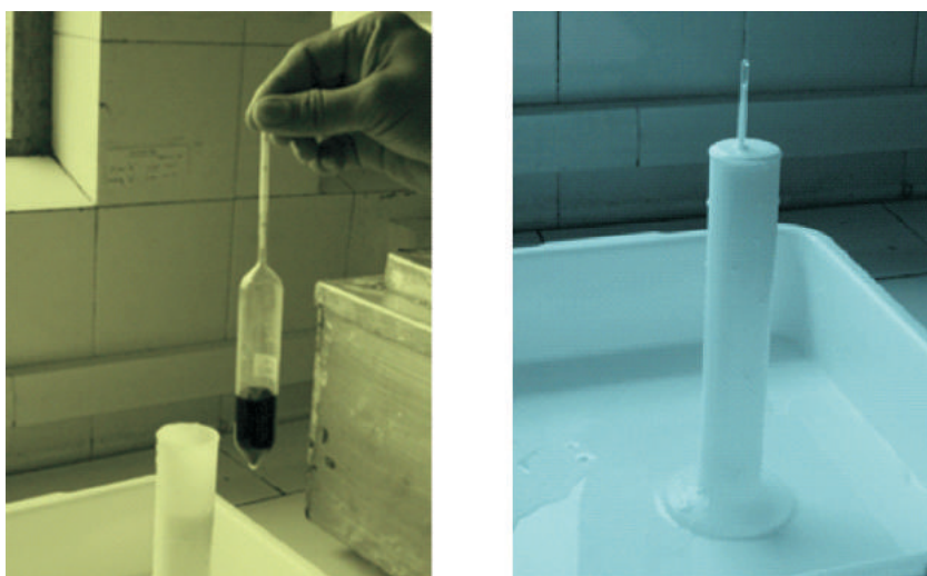
Fig.1.3. Determination of specific gravity of milk by ISI lactometer
