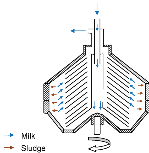
Fig.6.2. Clarifier
