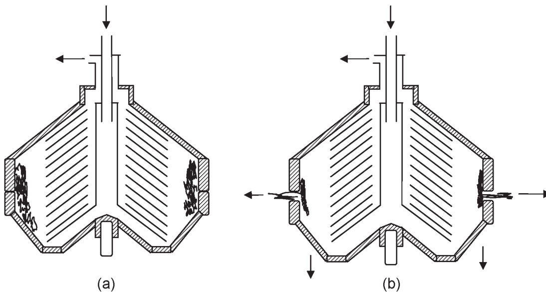
Fig. 6.3 Self desludging clarifier
