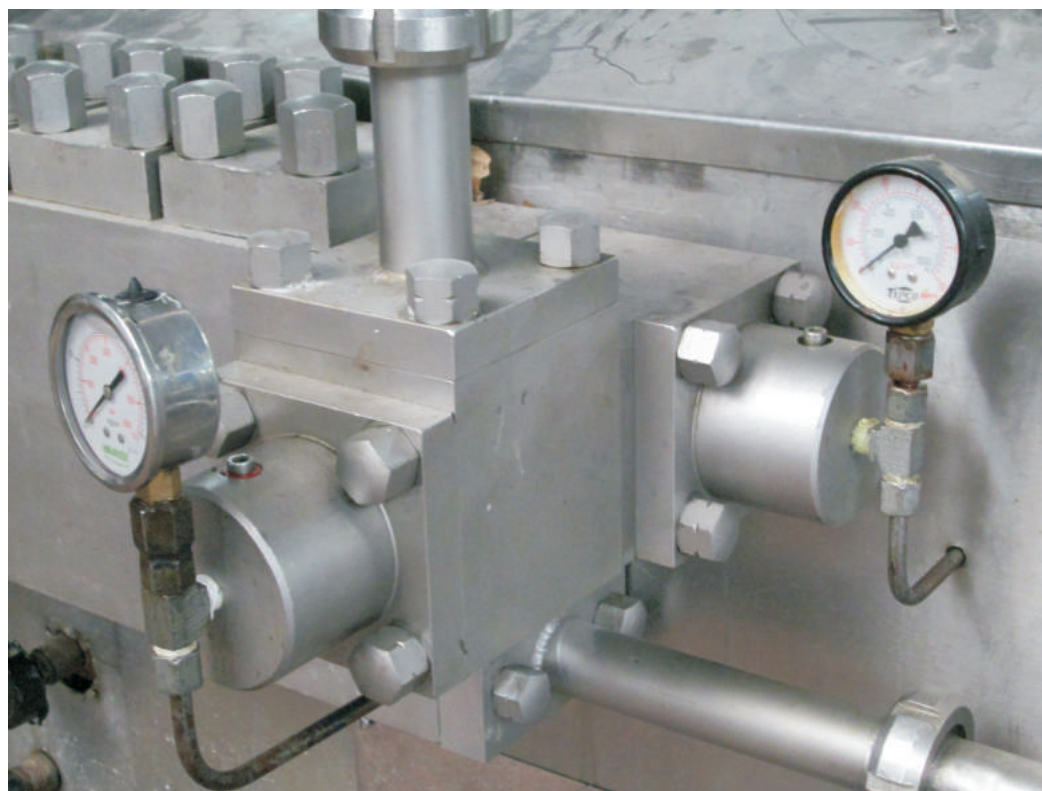
Fig.8.5. Pressure gauge
