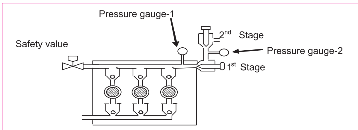
Fig.8.4. Milk homogenizer
