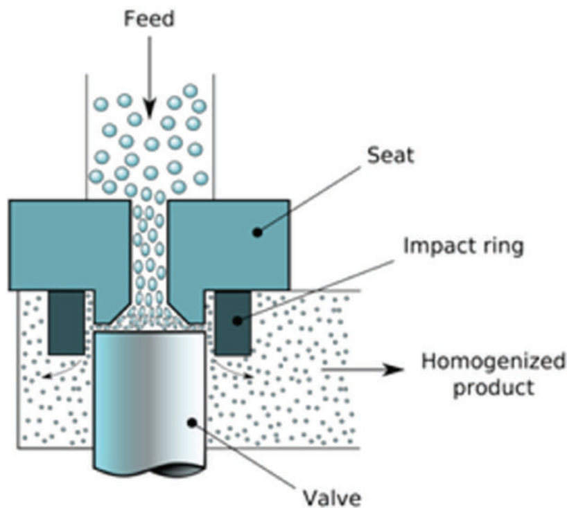
Fig.8.3. Homogenizer valve system
