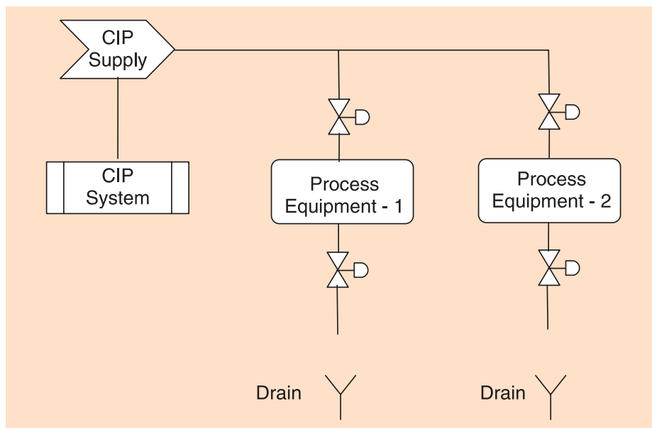
Fig.10.1. Single use CIP system
