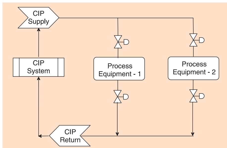
Fig.10.2. Re-use CIP system
