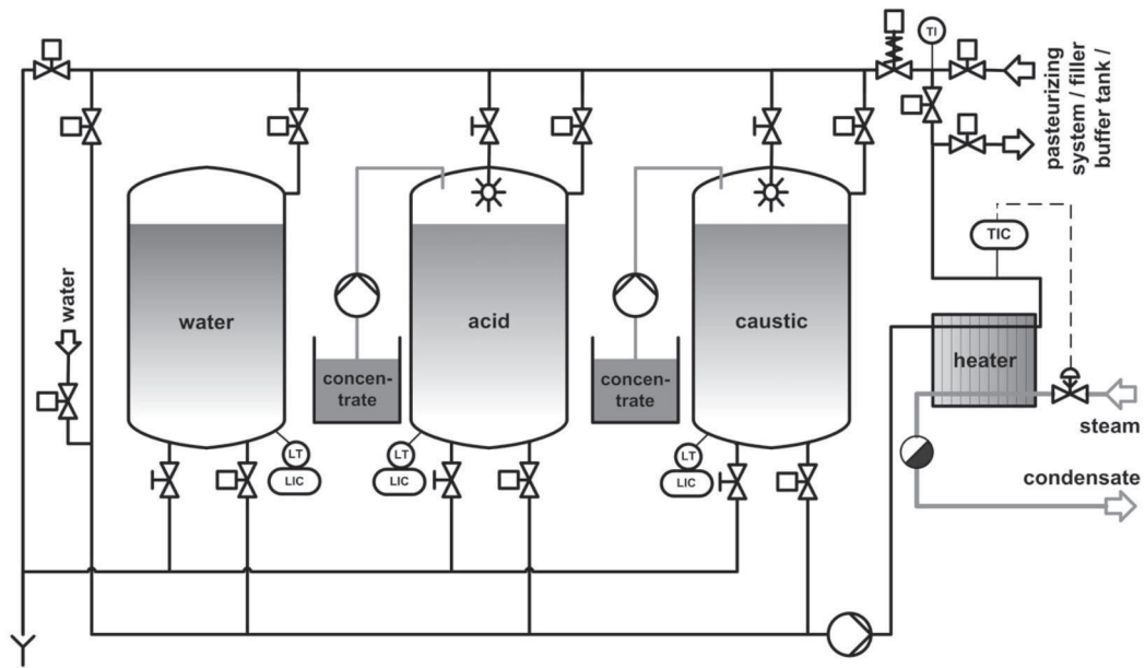
Fig.10.5. Components of a CIP system
