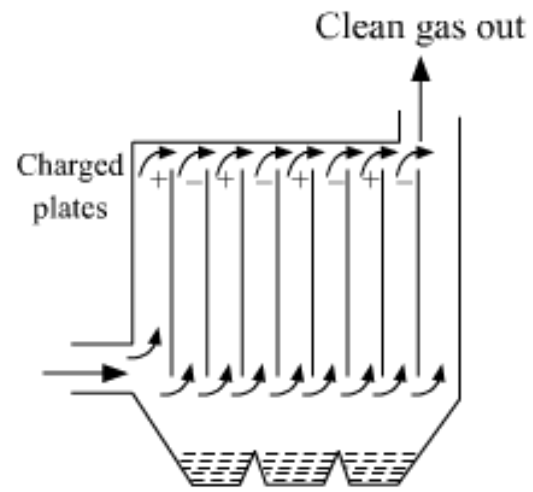
A plate type electrostatic precipitators
