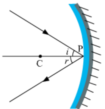
Concave mirror
