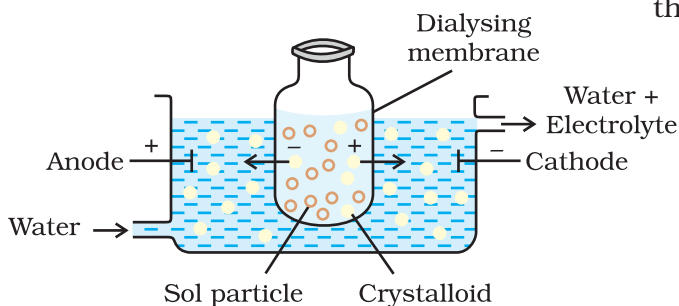
Fig. 5.10: Electro-dialysis
